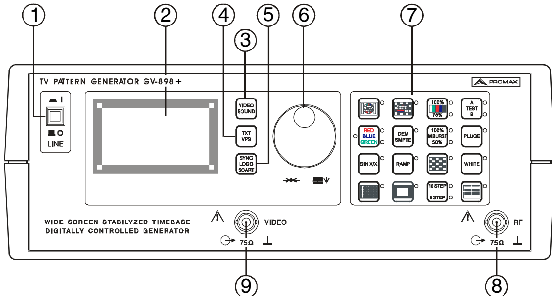
Figure 2.- Front panel
